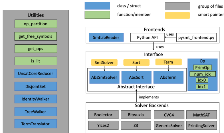
Fig. 1: Architecture diagram
